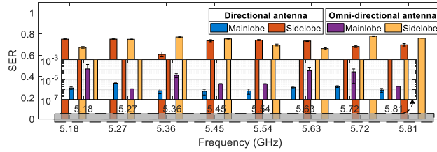
(b) Symbol error rate.
