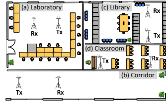
Figure 11: Deployment layout.
