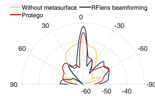
Figure 13: The performance of beamforming.
