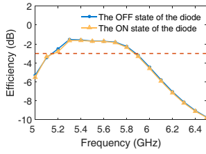
Figure 9: Simulated efficiency of metasurface.
