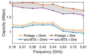
(a) Channel capacity.
