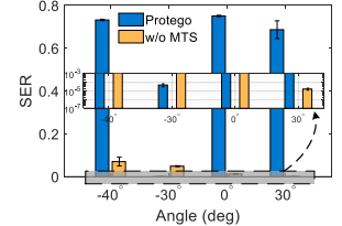
(c) Symbol error rate.
