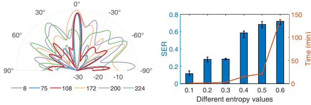
Figure 28: Beamwidth with different number of weak unit-cells. Figure 29: SER VS. time cost under different entropy values.
