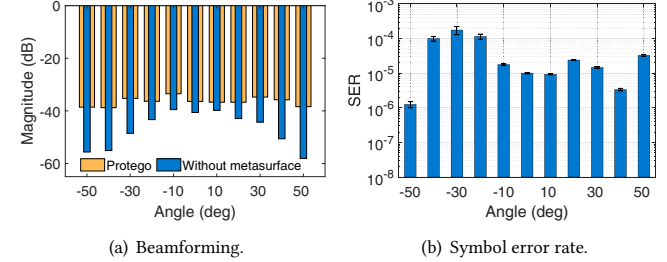
Figure 23: Impact of the legitimate user at different directions (i.e., [-50^\circ, 50^\circ] ).
