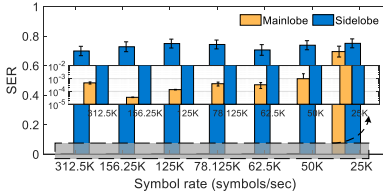
Figure 16: Experimental results of power improvement and SER at different operating frequencies.
