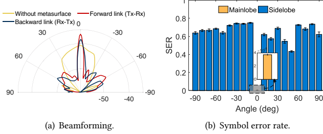
Figure 22: The beamforming and symbol error rate of backward link (i.e., receiver to transmitter).
